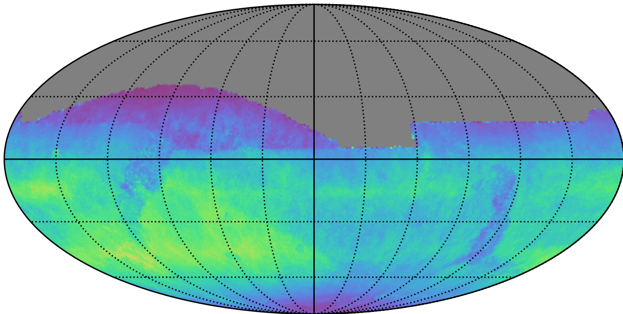
too_10_4v3.4_10yrs All sky z band: Normalized Teff
