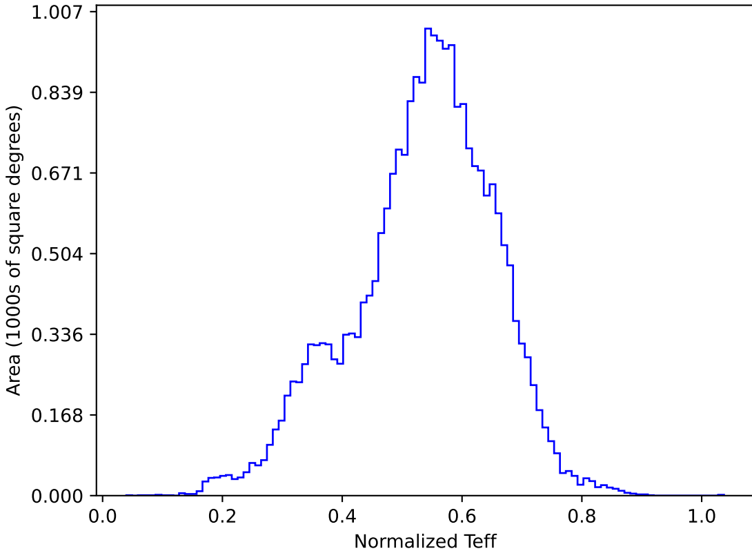
too_10_4v3.4_10yrs All sky y band: Normalized Teff
