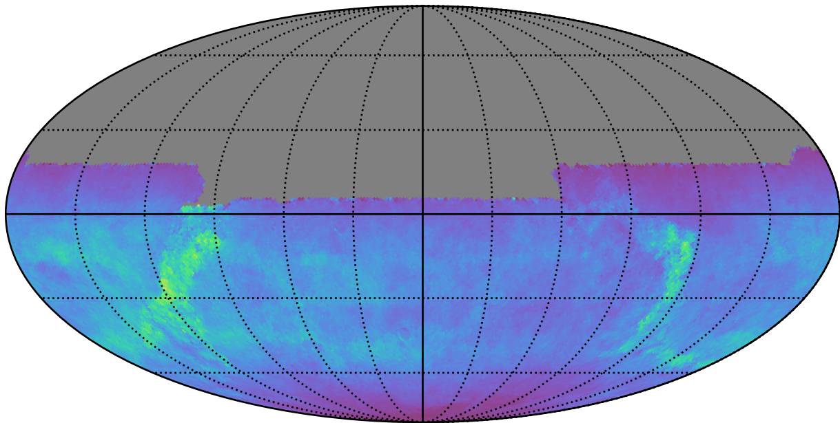
too_10_4v3.4_10yrs All sky u band: Normalized Teff
