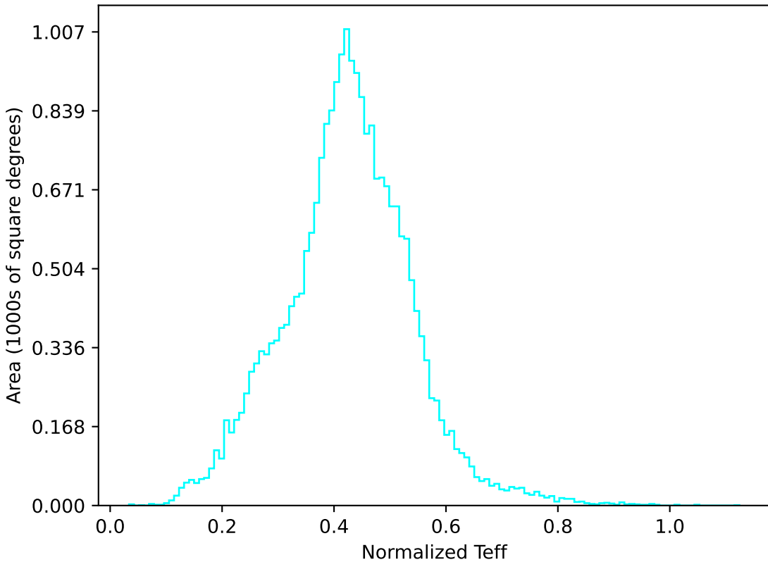
too_10_4v3.4_10yrs All sky u band: Normalized Teff
