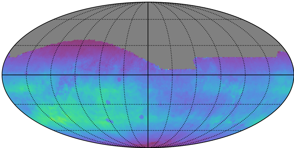
too_10_4v3.4_10yrs All sky r band: Normalized Teff
