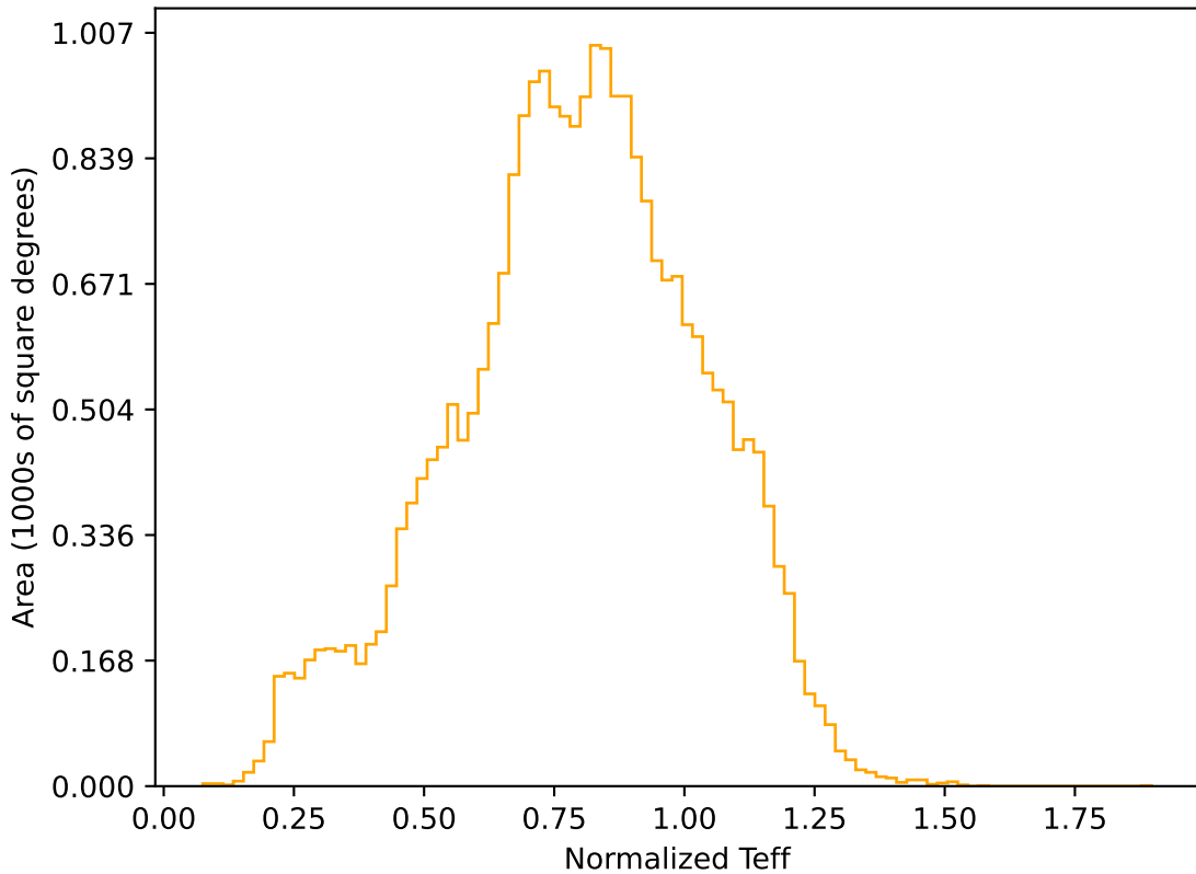
too_10_4v3.4_10yrs All sky r band: Normalized Teff
