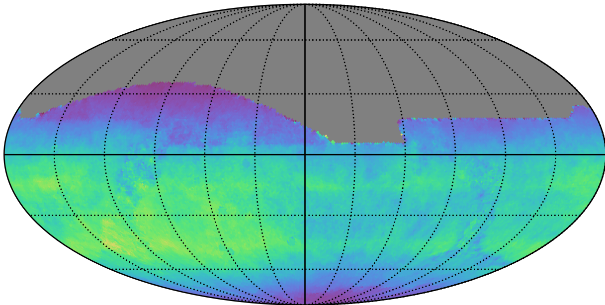
too_10_4v3.4_10yrs All sky i band: Normalized Teff
