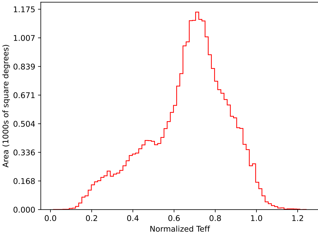
too_10_4v3.4_10yrs All sky i band: Normalized Teff
