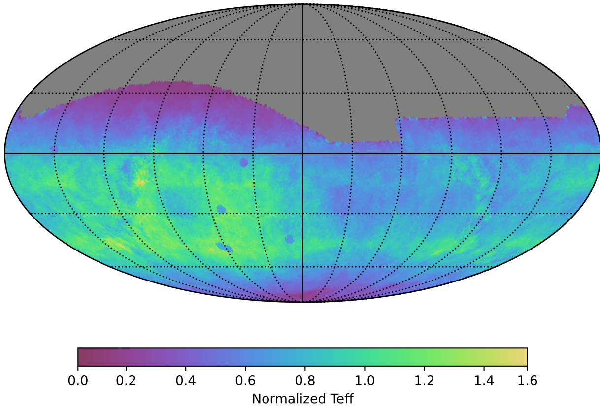
too_10_4v3.4_10yrs All sky g band: Normalized Teff
