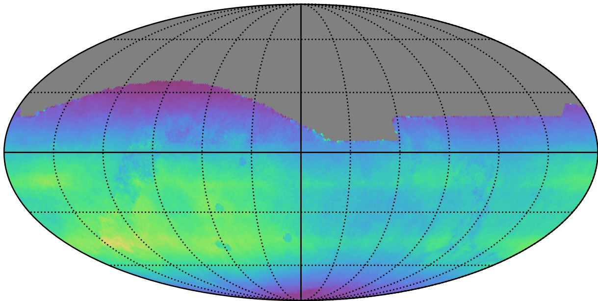
too_10_4v3.4_10yrs All sky all bands: Normalized Teff
