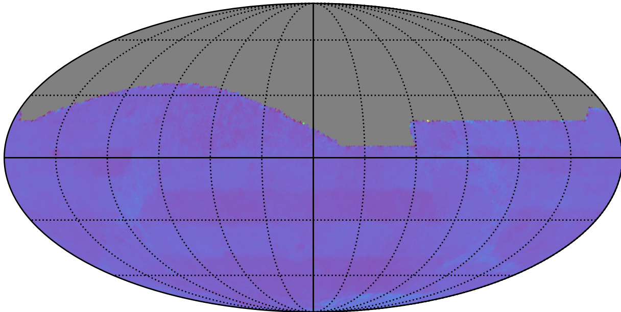
too_10_4v3.4_10yrs All sky: Normalized Proper Motion Uncert @ 24.0
