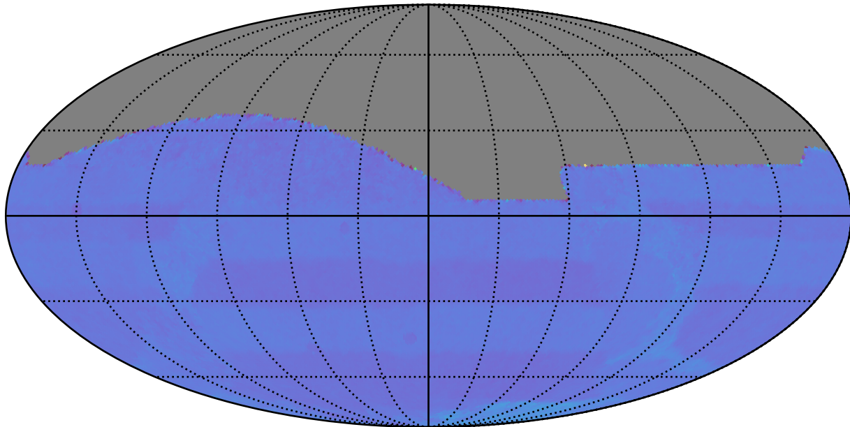
too_10_4v3.4_10yrs All sky: Normalized Proper Motion Uncert @ 20.5
