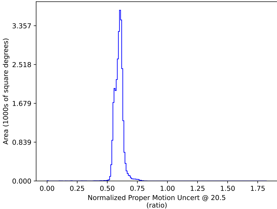
too_10_4v3.4_10yrs All sky: Normalized Proper Motion Uncert @ 20.5
