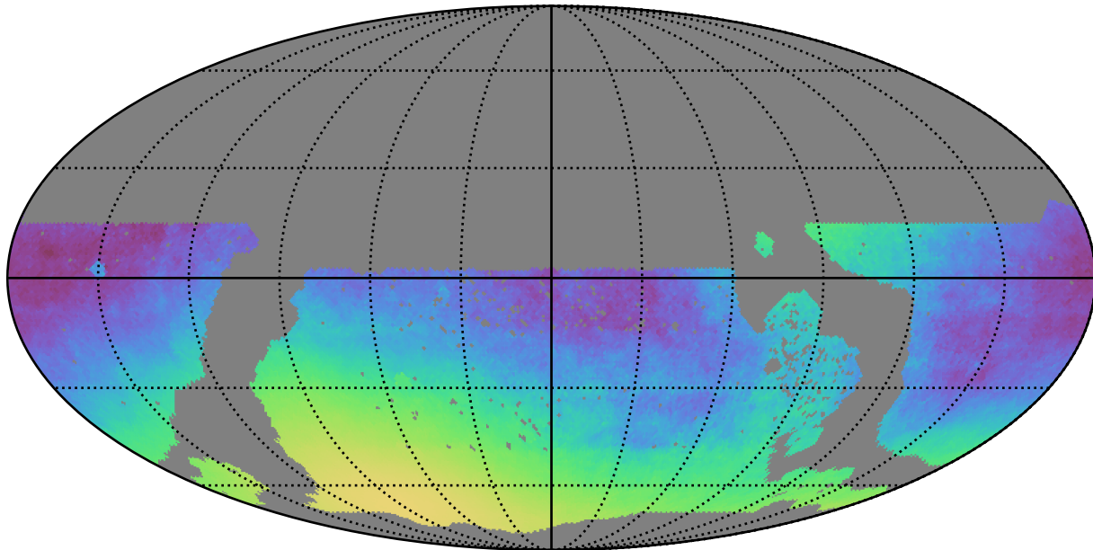
too_10_4v3.4_10yrs WFD: Normalized Parallax Uncert @ 24.0
