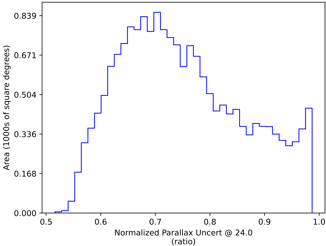
too_10_4v3.4_10yrs WFD: Normalized Parallax Uncert @ 24.0
