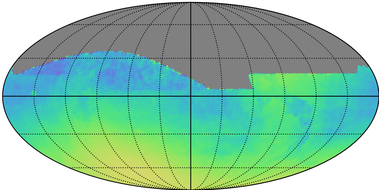
too_10_4v3.4_10yrs All sky: Normalized Parallax Uncert @ 24.0
