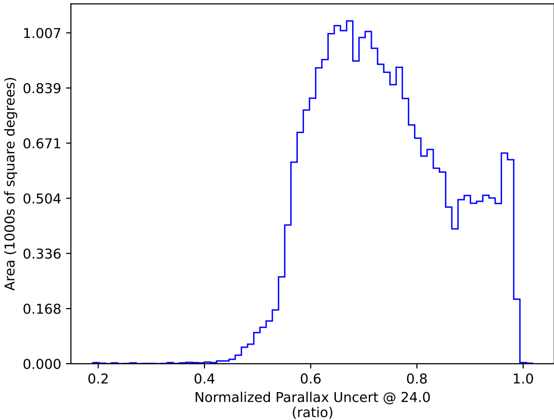
too_10_4v3.4_10yrs All sky: Normalized Parallax Uncert @ 24.0
