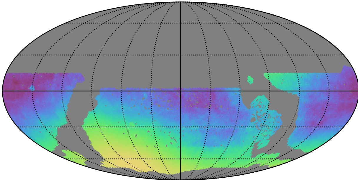
too_10_4v3.4_10yrs WFD: Normalized Parallax Uncert @ 22.4
