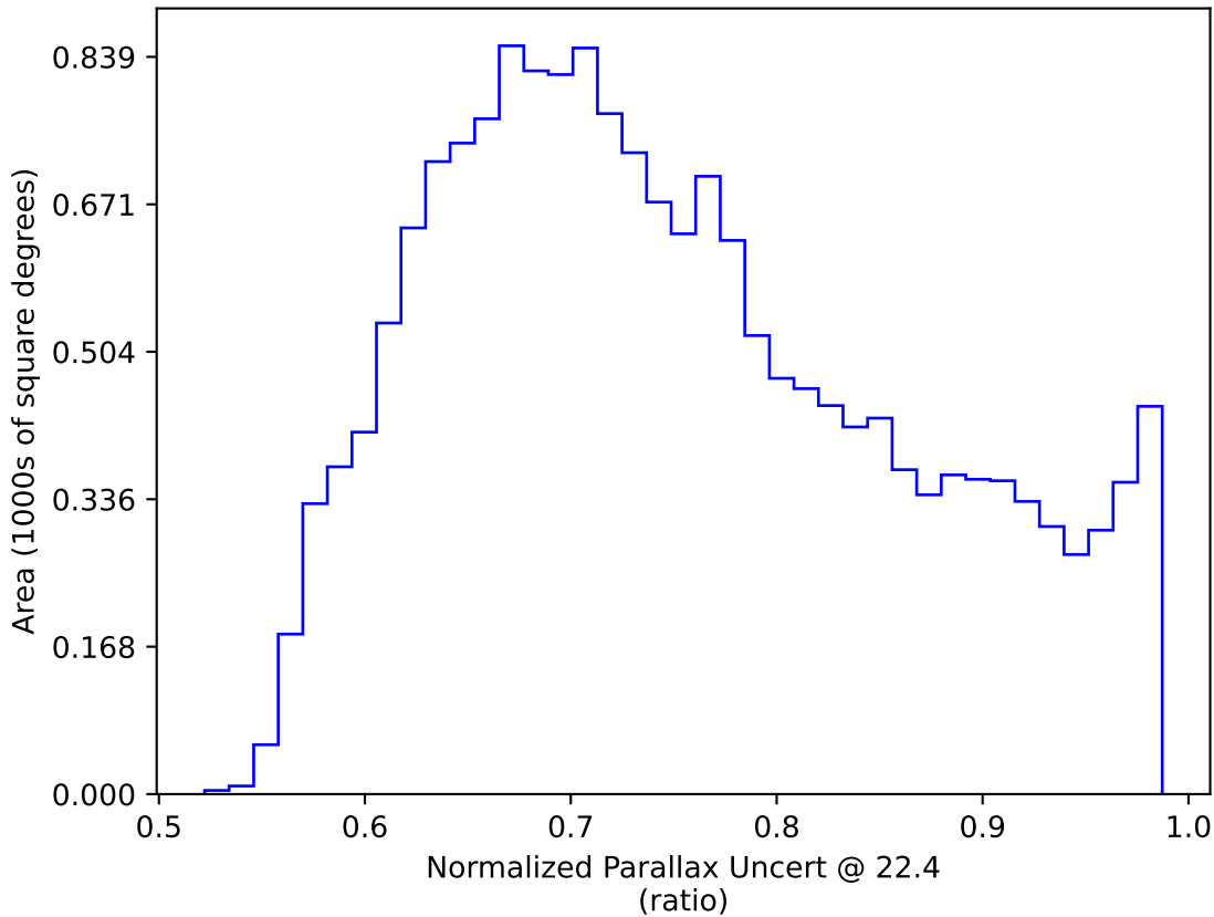
too_10_4v3.4_10yrs WFD: Normalized Parallax Uncert @ 22.4
