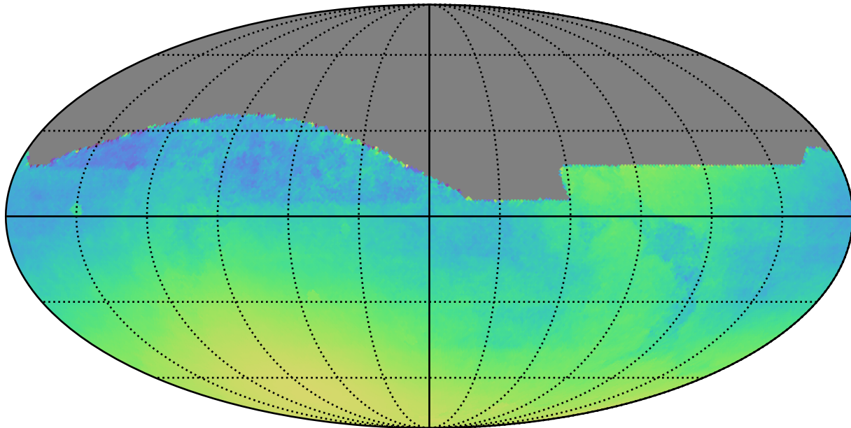
too_10_4v3.4_10yrs All sky: Normalized Parallax Uncert @ 22.4
