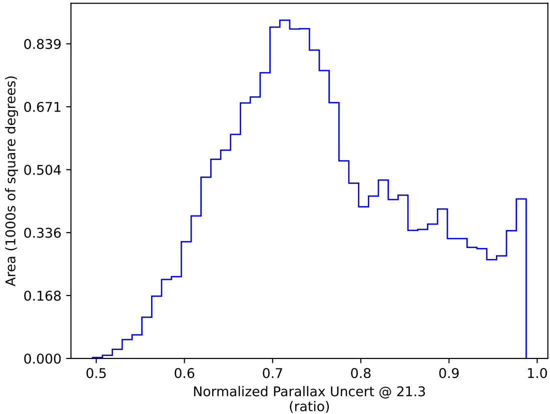
too_10_4v3.4_10yrs WFD y band only: Normalized Parallax Uncert @ 21.3
