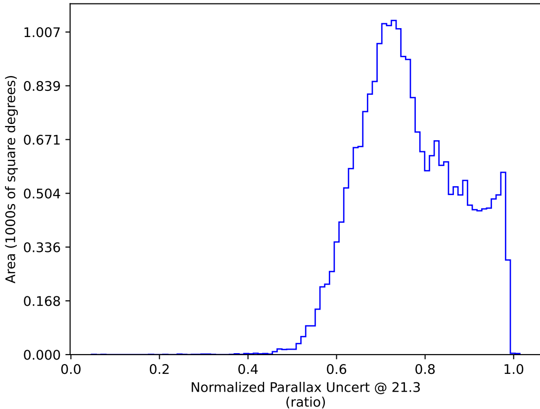
too_10_4v3.4_10yrs All sky y band only: Normalized Parallax Uncert @ 21.3
