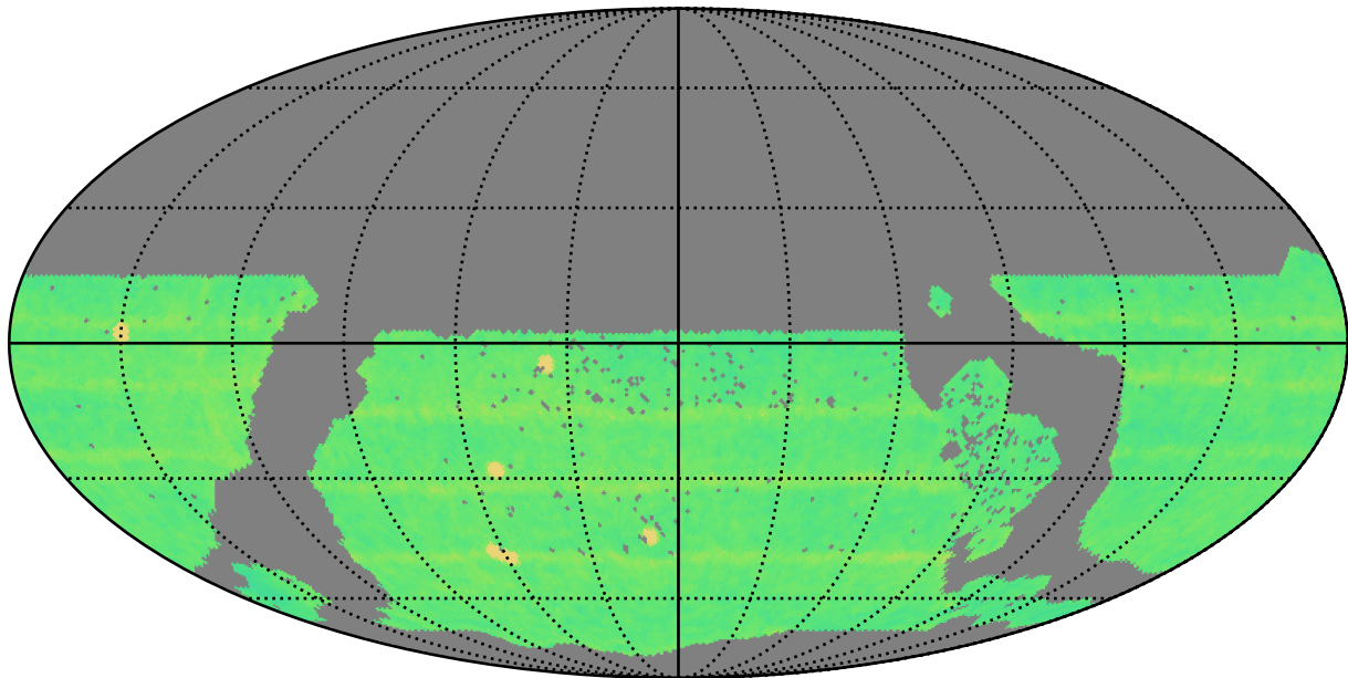
too_10_4v3.4_10yrs WFD all bands: N Unique Nights
