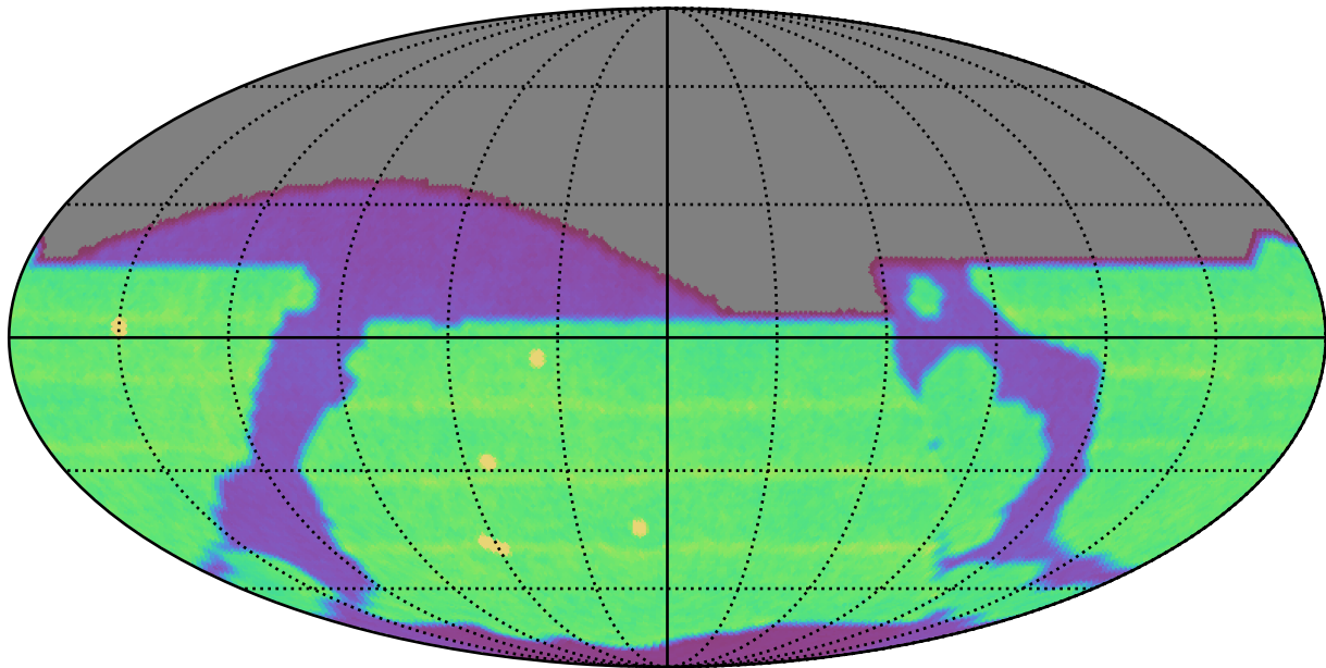
too_10_4v3.4_10yrs All sky all bands: N Unique Nights
