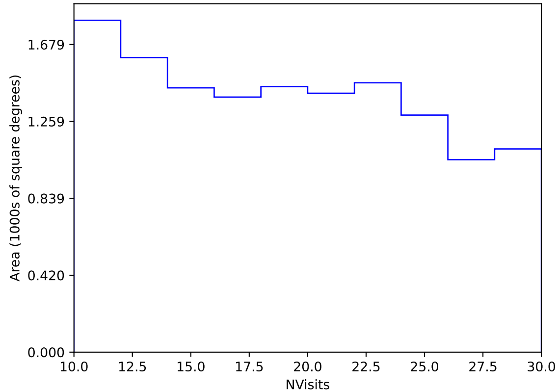
too_10_4v3.4_10yrs Yr 3-4 y band: NVisits
