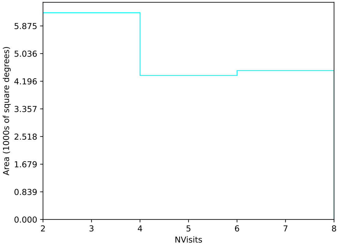
too_10_4v3.4_10yrs Yr 3-4 u band: NVisits
