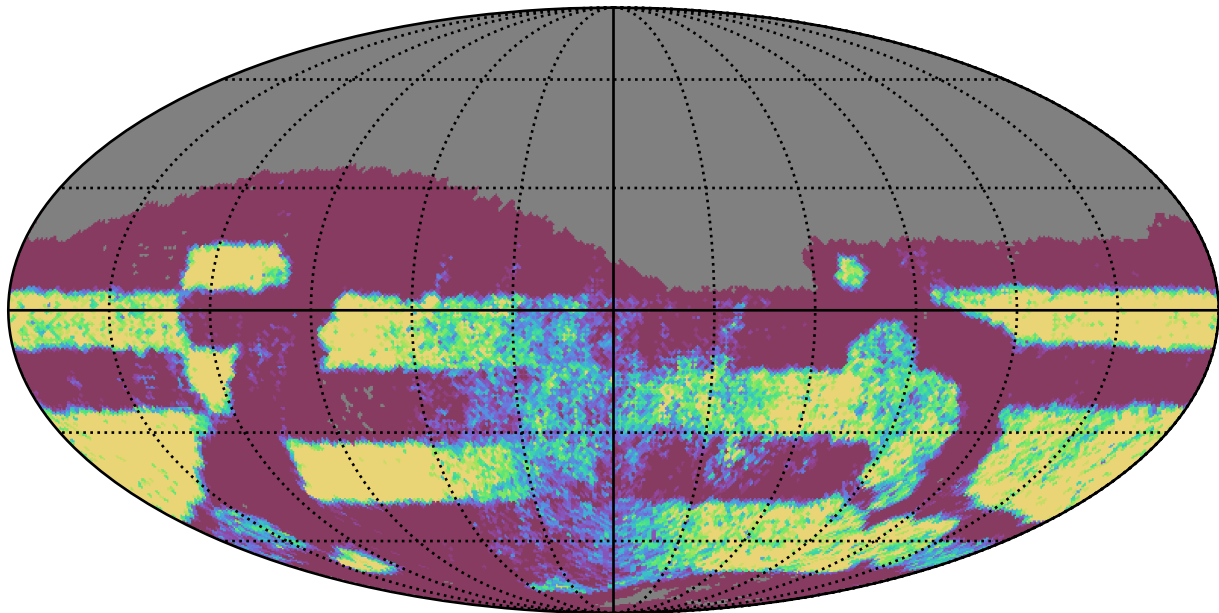
too_10_4v3.4_10yrs Yr 3-4 r band: NVisits
