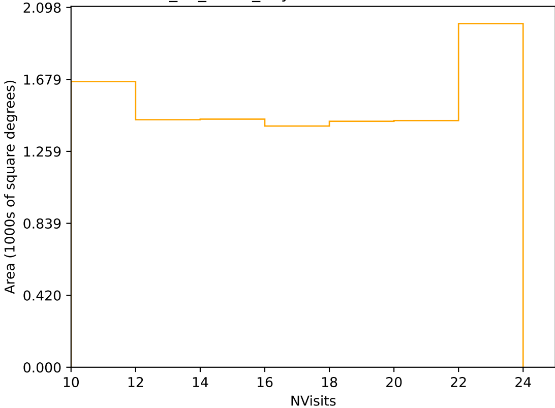
too_10_4v3.4_10yrs Yr 3-4 r band: NVisits
