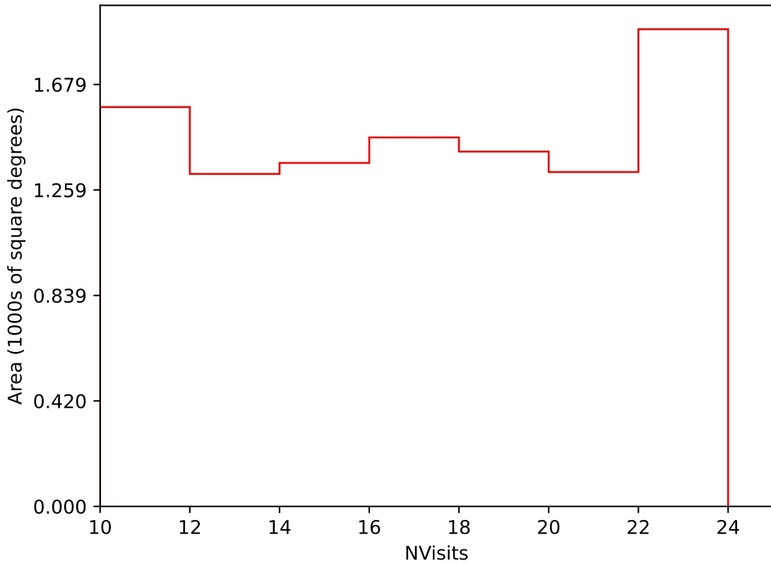
too_10_4v3.4_10yrs Yr 3-4 i band: NVisits
