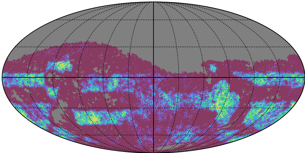
too_10_4v3.4_10yrs Yr 3-4 g band: NVisits
