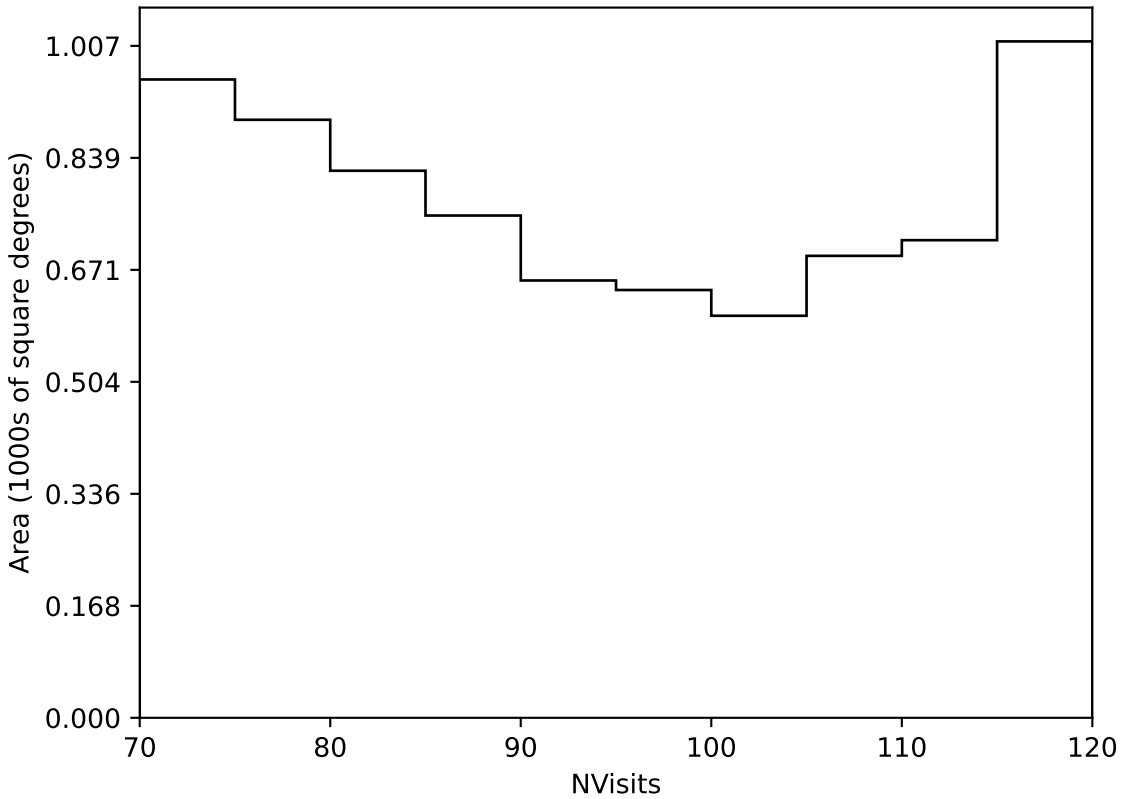
too_10_4v3.4_10yrs Yr 3-4 all bands: NVisits
