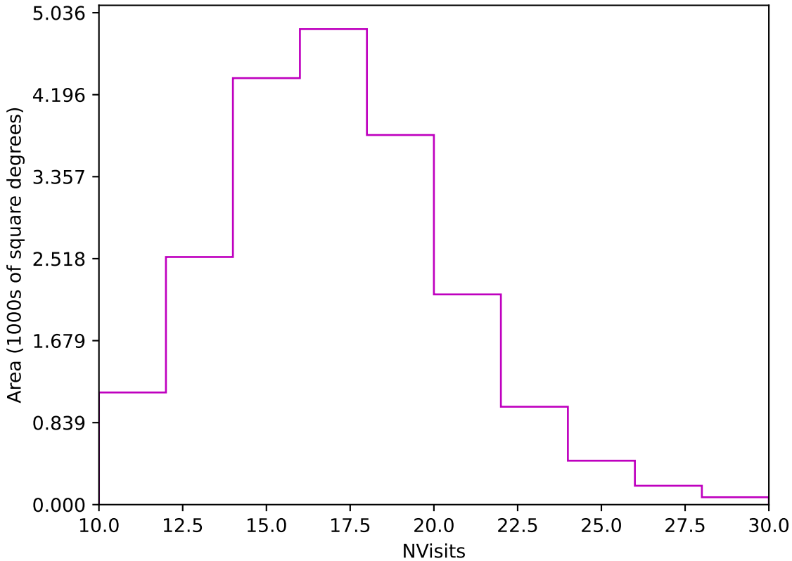
too_10_4v3.4_10yrs Yr 1 z band: NVisits
