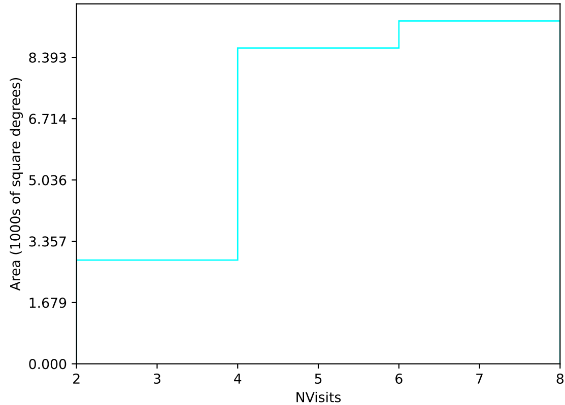
too_10_4v3.4_10yrs Yr 1 u band: NVisits
