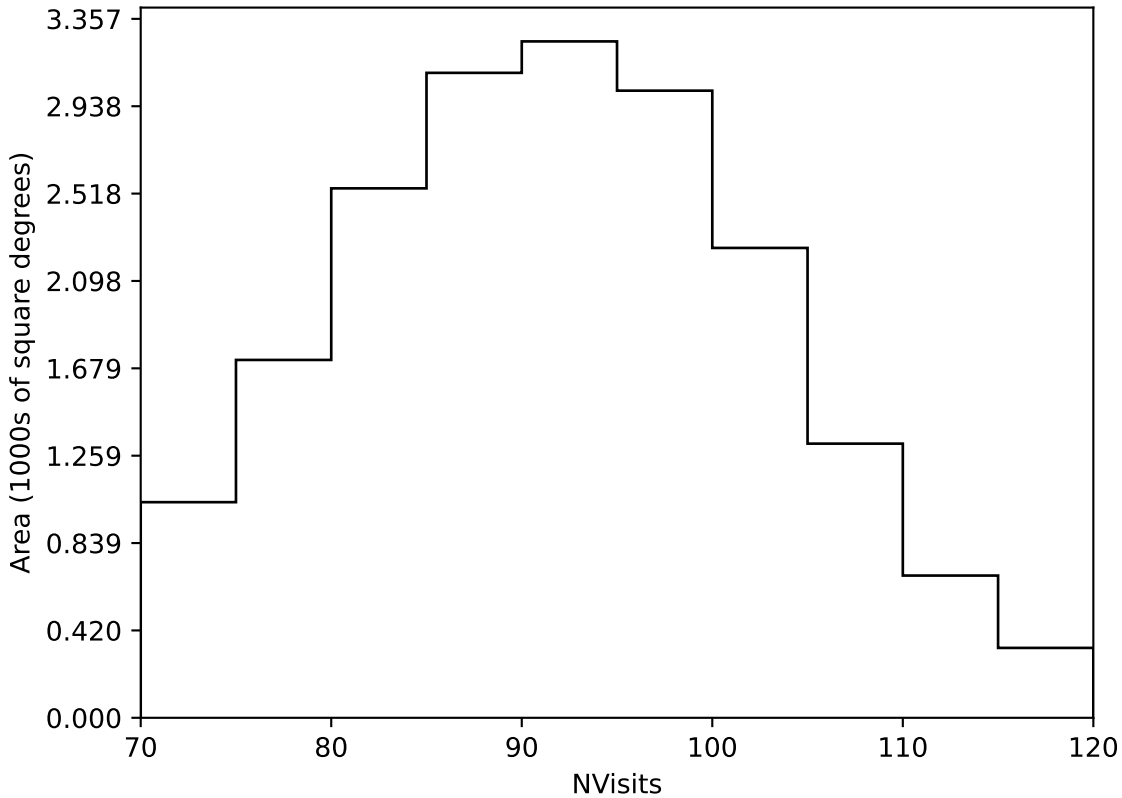
too_10_4v3.4_10yrs Yr 1 all bands: NVisits
