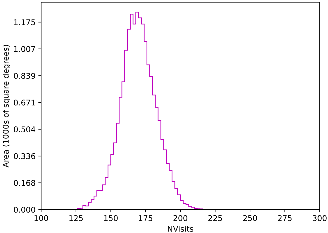
too_10_4v3.4_10yrs WFD z band: NVisits
