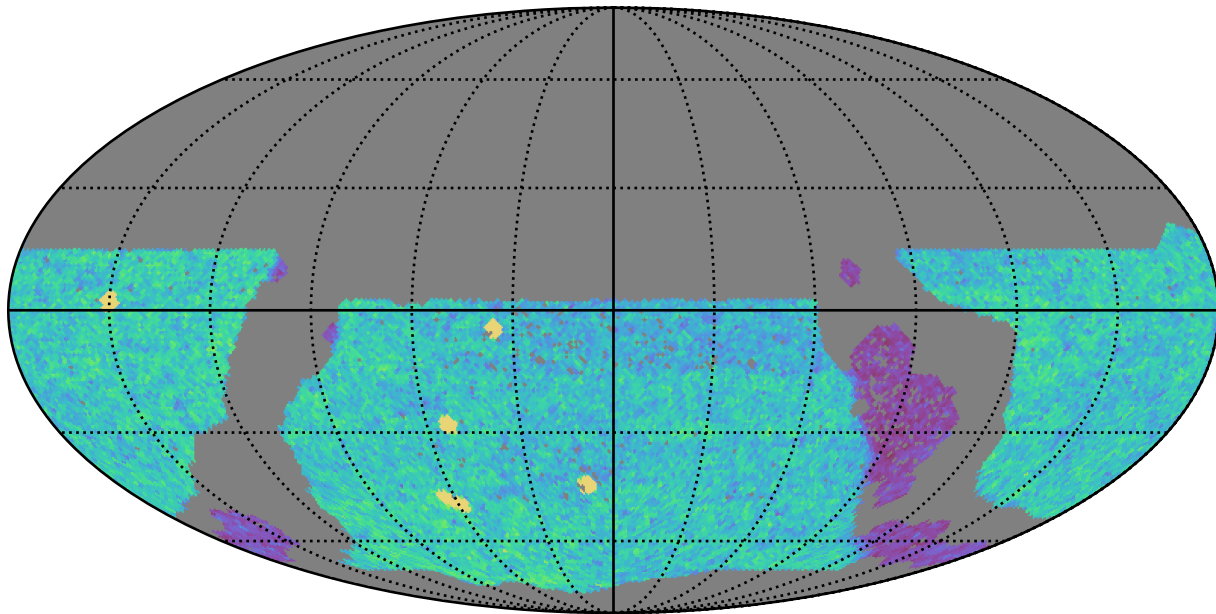
too_10_4v3.4_10yrs WFD u band: NVisits
