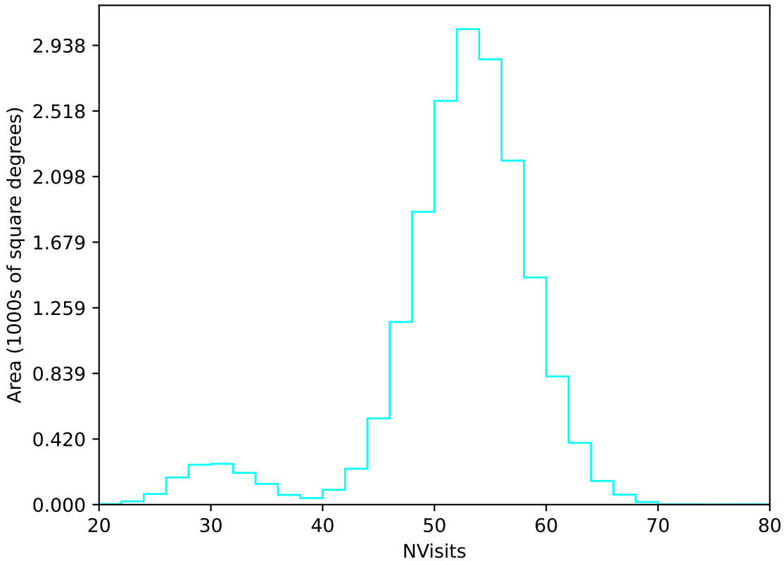
too_10_4v3.4_10yrs WFD u band: NVisits
