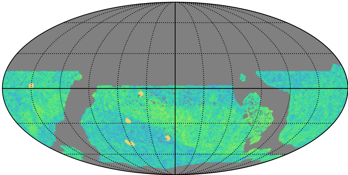
too_10_4v3.4_10yrs WFD i band: NVisits
