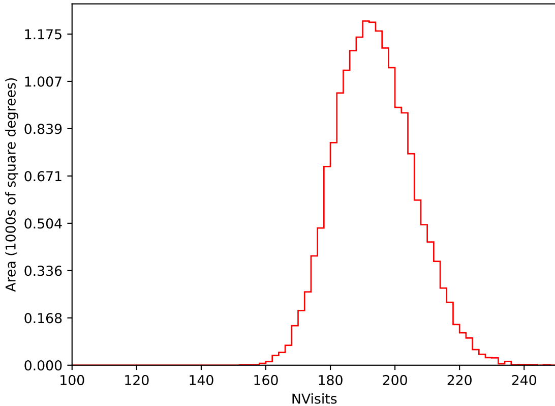
too_10_4v3.4_10yrs WFD i band: NVisits
