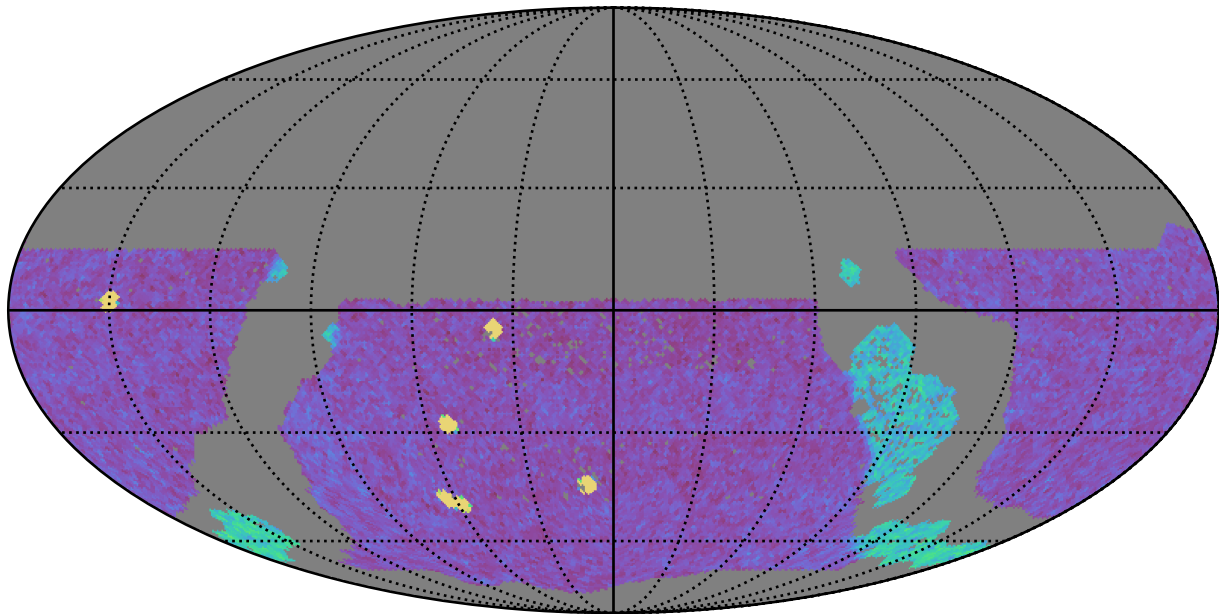
too_10_4v3.4_10yrs WFD g band: NVisits
