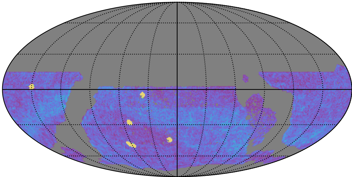
too_10_4v3.4_10yrs WFD all bands: NVisits
