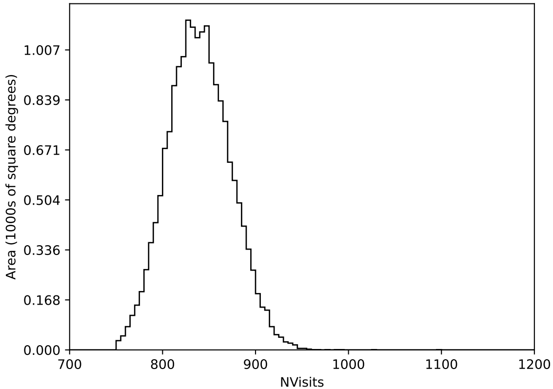
too_10_4v3.4_10yrs WFD all bands: NVisits
