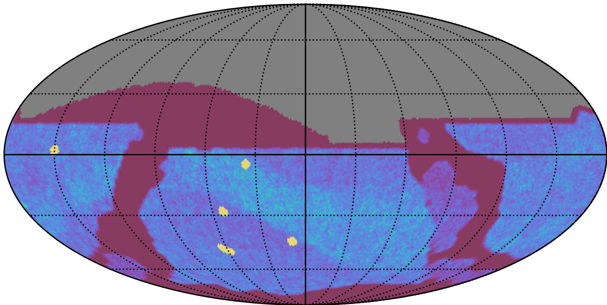
too_10_4v3.4_10yrs All sky z band: NVisits
