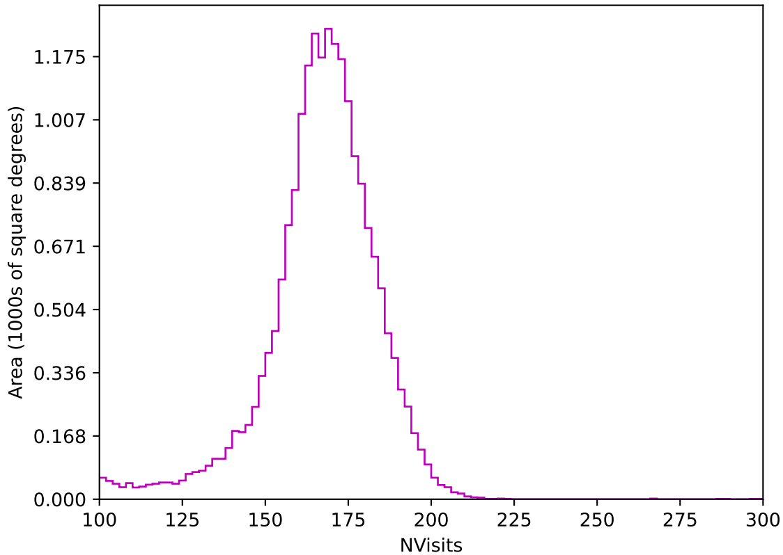
too_10_4v3.4_10yrs All sky z band: NVisits
