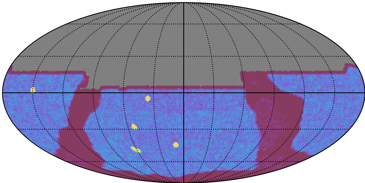
too_10_4v3.4_10yrs All sky y band: NVisits
