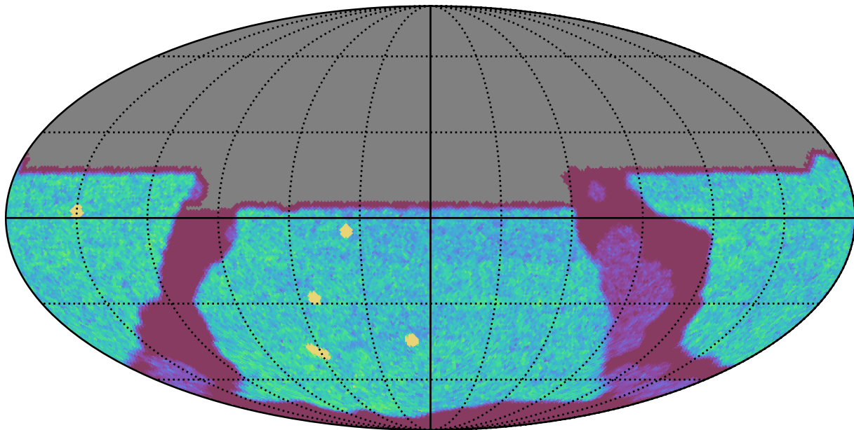
too_10_4v3.4_10yrs All sky u band: NVisits
