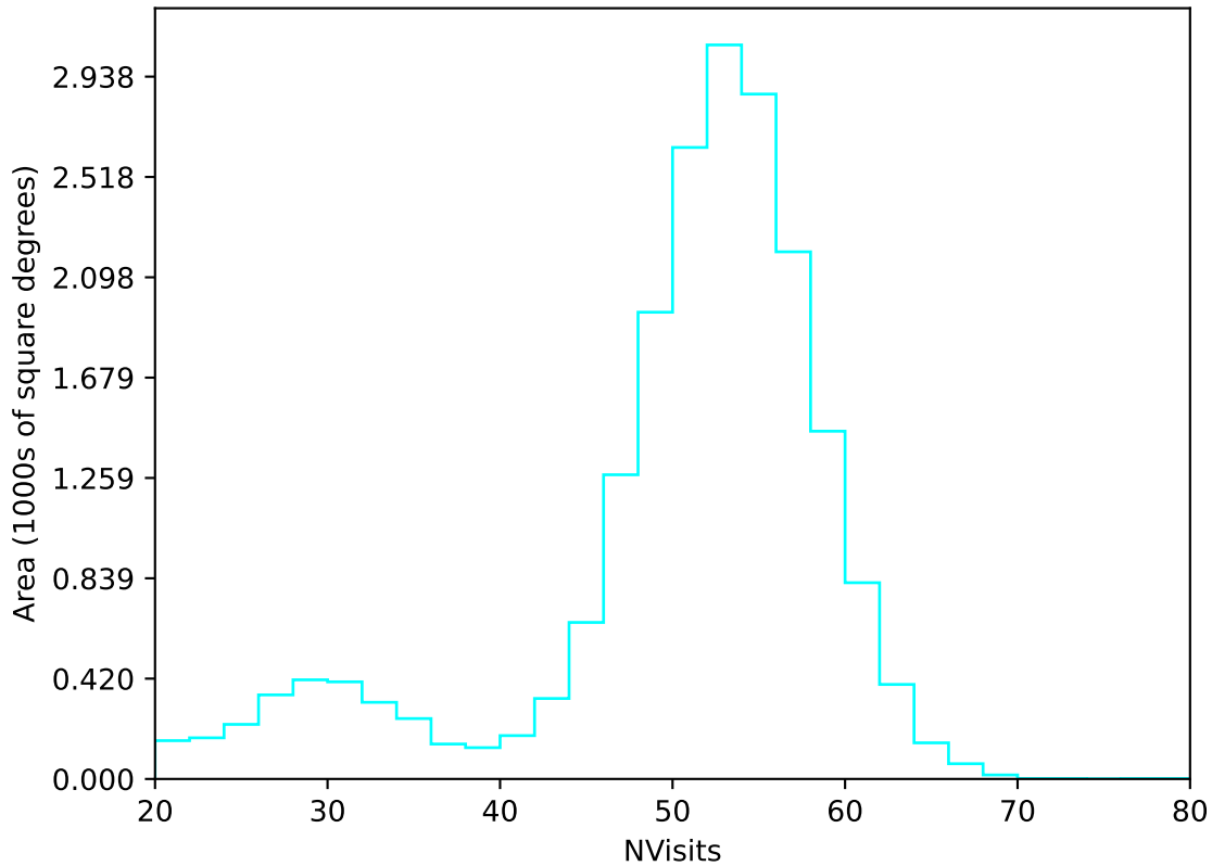
too_10_4v3.4_10yrs All sky u band: NVisits
