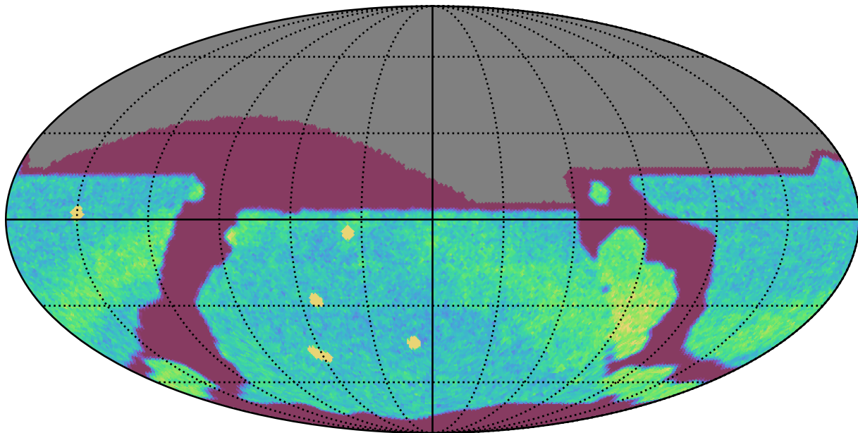
too_10_4v3.4_10yrs All sky r band: NVisits
