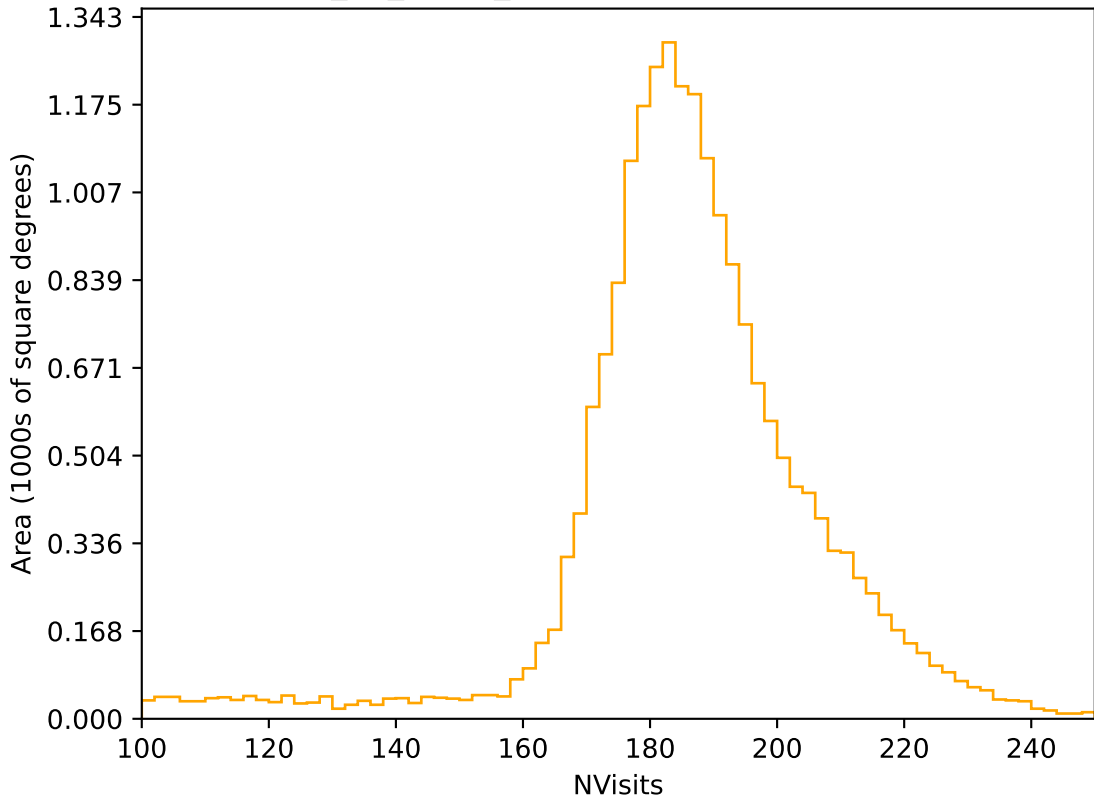
too_10_4v3.4_10yrs All sky r band: NVisits
