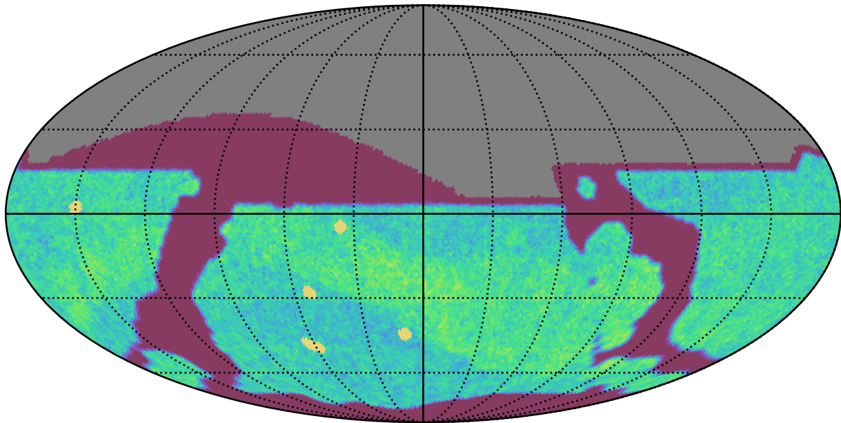
too_10_4v3.4_10yrs All sky i band: NVisits
